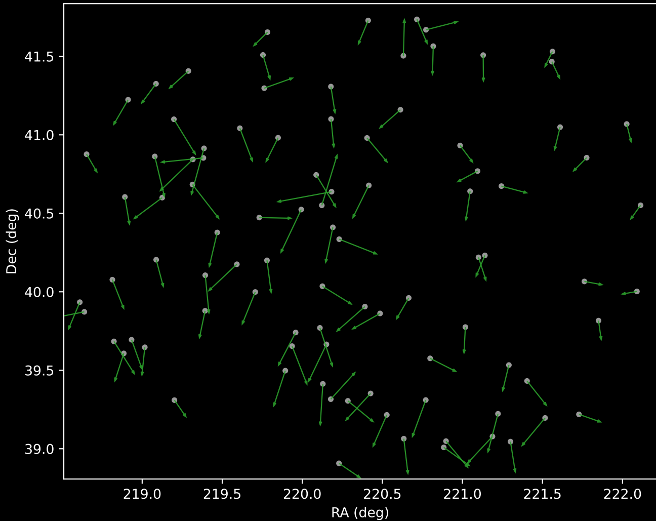
APOGEE DR17 Cluster 4 Proper Motion Vectors (n=93)
