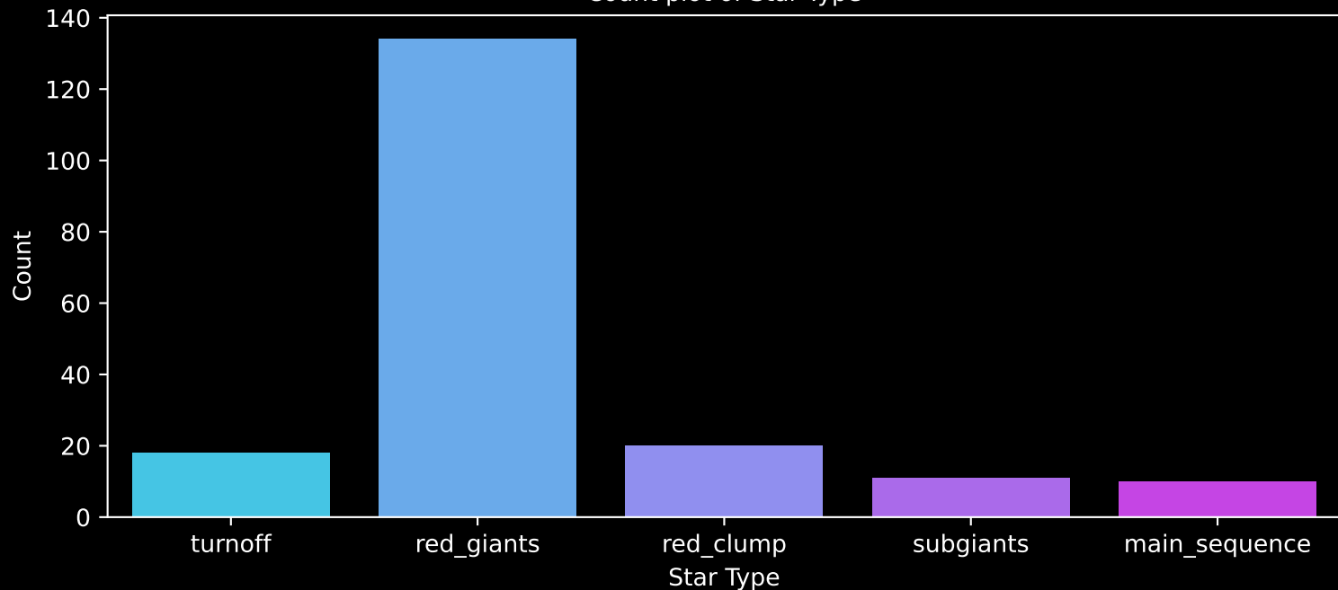
APOGEE DR17 Field: [180+30] Count plot of Star Type
