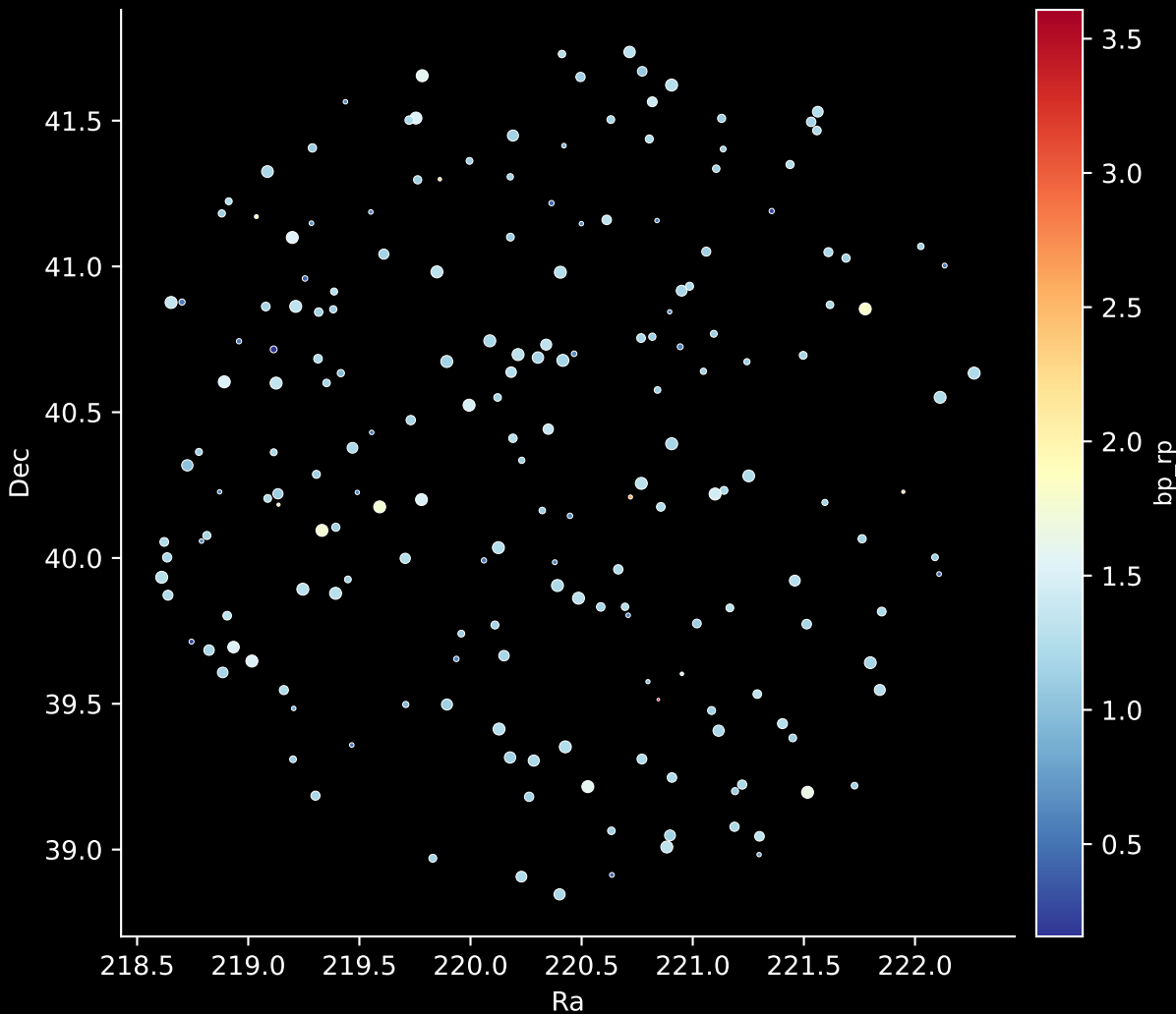
APOGEE DR17 Field: [180+30] Stars: 193
