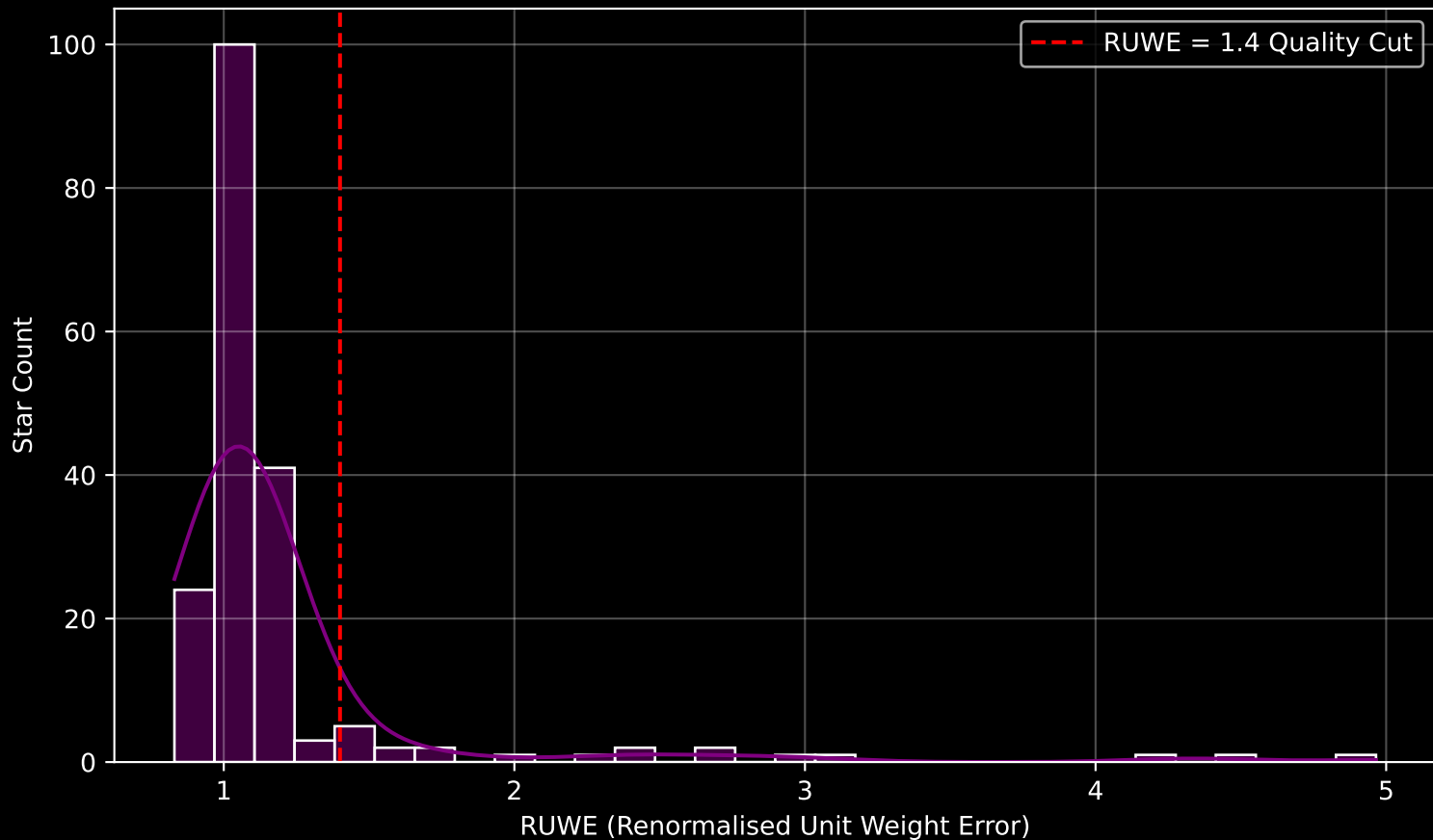
GAPOGEE DR17 Field [180+30] RUWE Distribution (n= 188)
