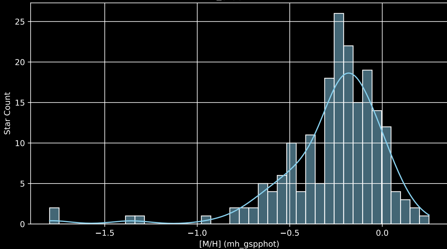
APOGEE DR17 Field: [180+30 [M/H] (mh_gspphot) (n= 192)
