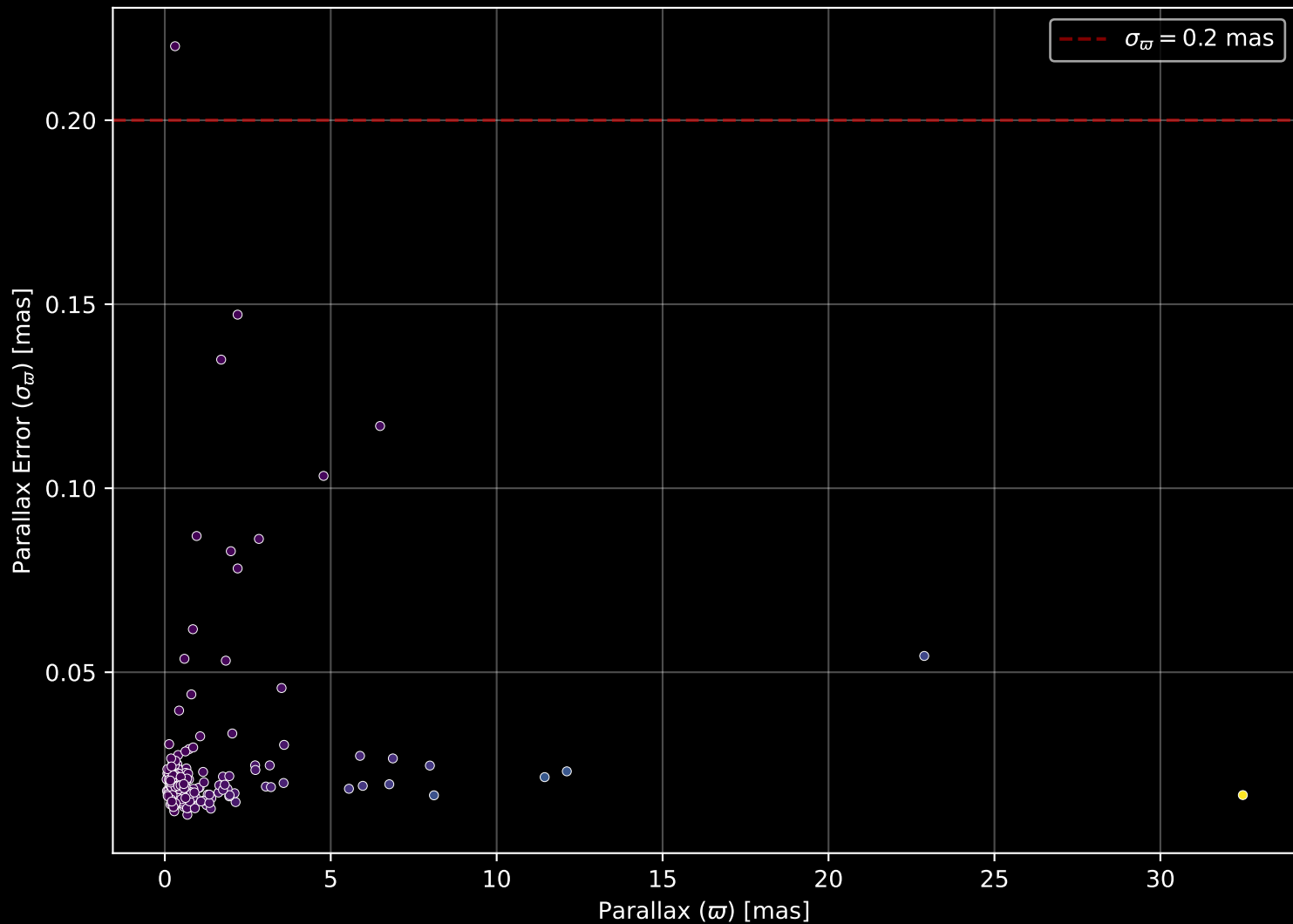
APOGEE DR17 Field: [180+30] Parallax Quality (n= 193)
