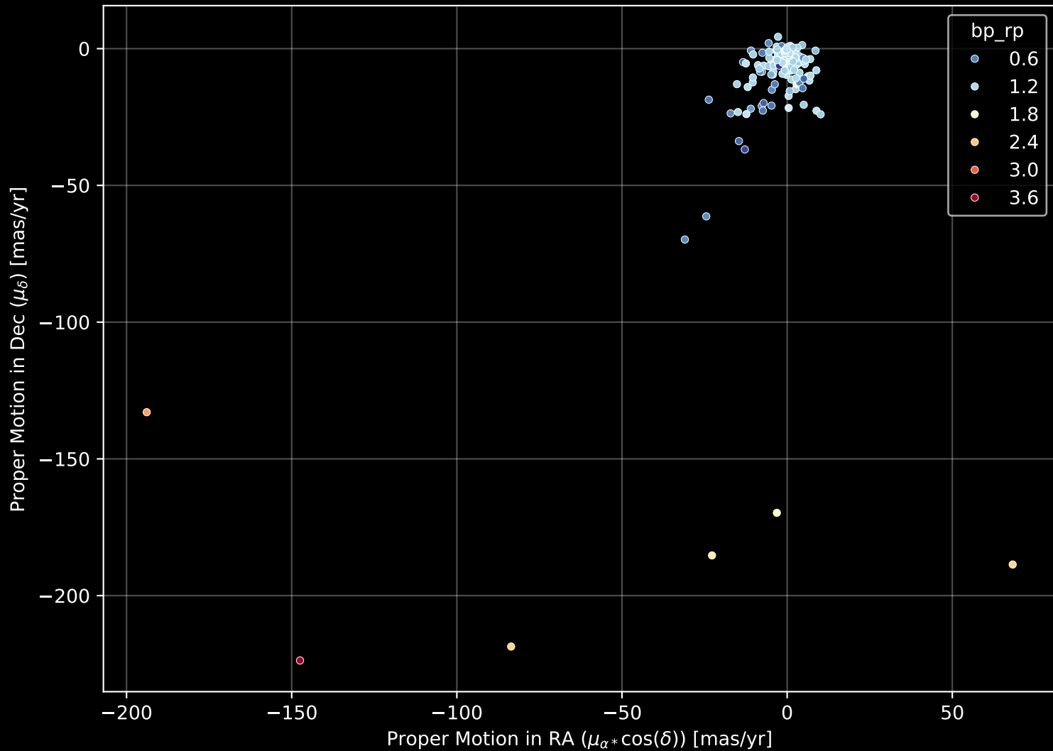
APOGEE DR17 Field: [180+30] Proper Motion Diagram (n= 193)
